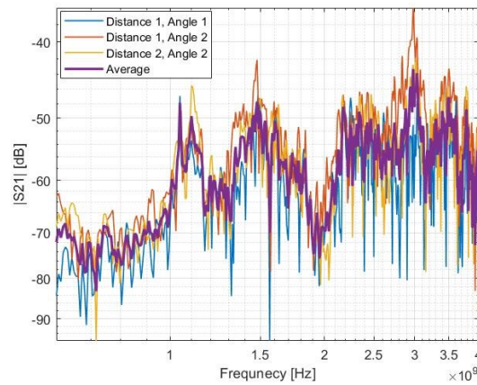
Fig. 6. |S_{21}| values in three cases using different settings in each case
