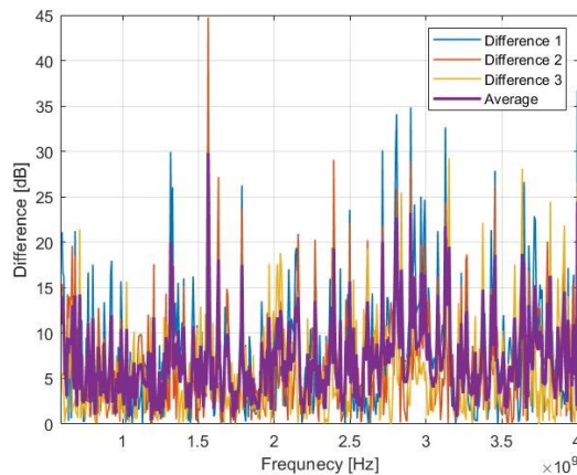
Fig. 8. Calculated difference between the source and the victim in three cases using different settings in each case
