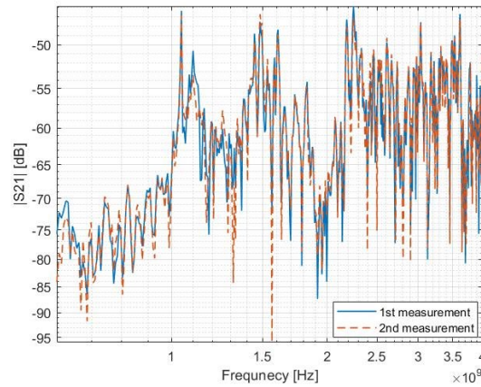
Fig. 5. |S_{21}| values using the same setup but measured at different times
