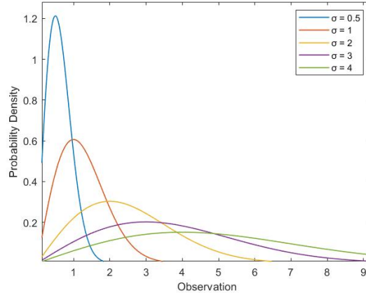
Fig. 9. Rayleigh Distribution for different mode values ( \sigma )
