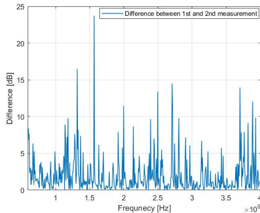
Fig. 7. Calculated difference between the source and the victim using the same setup but measured at different times
