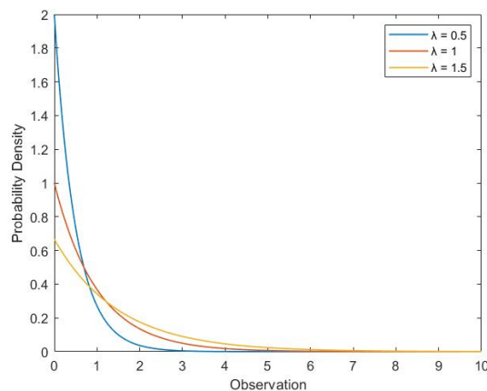
Fig. 10. Exponential Distribution for different mean values ( 1/\lambda )
