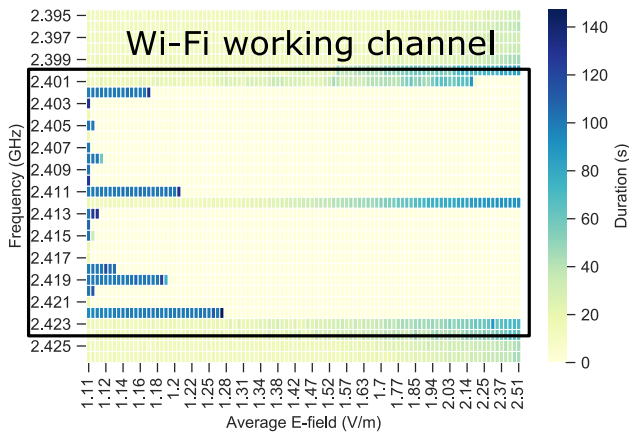
Fig. 5: RC1. Packet transmission time heatmap depending on CW EMD values
