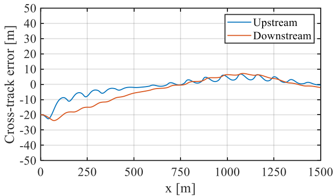
FIGURE 10: CROSS-TRACK ERROR RESULT.
