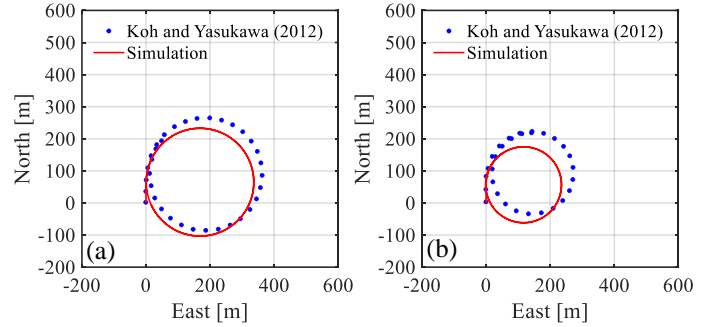
FIGURE 4: MODEL VERIFICATION ON TURNING: (a) \delta = 35^\circ , AND (b) \delta = 20^\circ .
