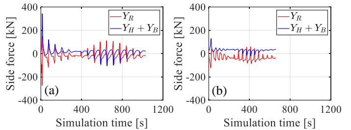
FIGURE 8: TIME HISTORIES OF SIDE FORCE (a) UPSTREAM CURRENT, AND (b) DOWNSTREAM CURRENT.
