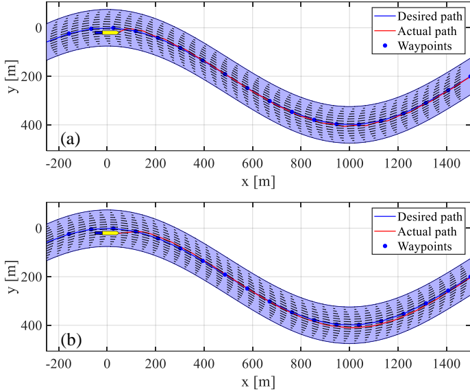
FIGURE 6: IWV TRAJECTORY OF MID-CHANNEL SAILING: (a) UPSTREAM CURRENT, AND (b) DOWNSTREAM CURRENT.
