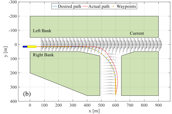
FIGURE 11: SIMULATION RESULTS FROM TURNING TRAJECTORY SIMULATIONS: (a) UPSTREAM CURRENT, AND (b) DOWNSTREAM CURRENT.
